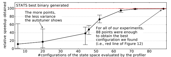
Figure 20. Average performance (geo. mean) of the binary found by the STATS autotuner after a number of configurations explored.
