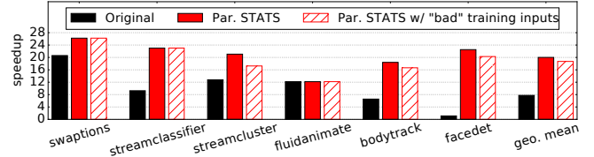
Figure 19. STATS loses only a small amount of performance when not representative inputs are used.
